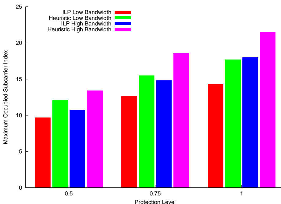
Figure 5.3 Maximum occupied subcarrier index of SPP and MPP schemes for ILP and heuristic algorithms.
